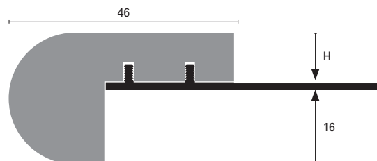
Illustrated scale dimension 1:1 (FW 100*)
